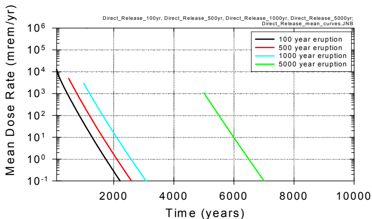
Igneous Case Non-Probability Weighted Direct Release Mean Dose Time Histories
