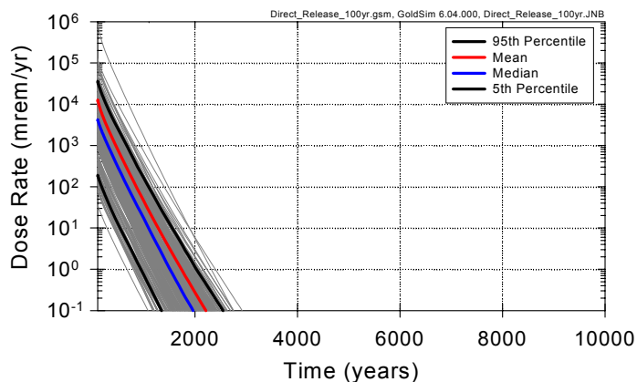
Igneous Case Non-Probability Weighted Direct Release Dose Time Histories Volcano Occurs at 100 Years
