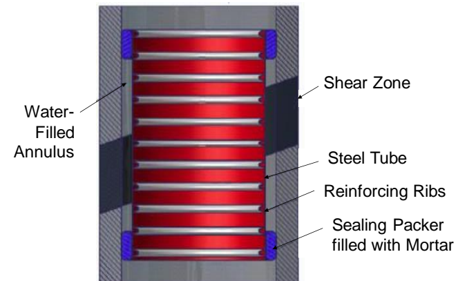
Surface Packer Schematic
